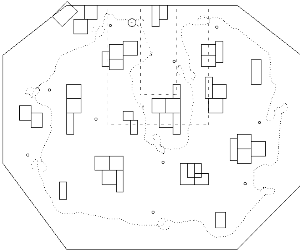
Figure 20: The dotted path traces the movements of Flakey during a partial run of Stage 2 for a simulated competition arena. Flakey started from the middle of the top wall heading left. Here, it has finished searching the perimeter of the arena and has just returned from its first foray (the dashed rectangle in the picture). CHECK-POLE maneuvers are visible near poles.
