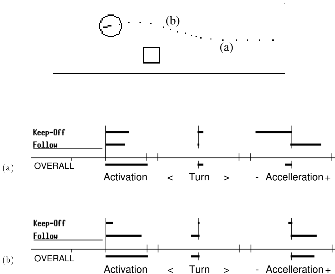
Figure 18: Flakey uses fuzzy rules to blend reactivity with purposeful action. In the top figure, Flakey moves from right to left. At location (a), an obstacle has been detected, and the preferences of KEEP-OFF are dominating; later, at location (b), the path is clear, and the goal-oriented preferences expressed by FOLLOW re-gain importance. The bars show the level of activation and the preferred controls for each behavior, and the result of the blending.
