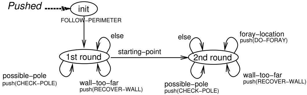
Figure 19: The tasks used by Flakey are finite-state machines. The EXPLORE task, is illustrated here; state transitions are labelled by the triggering perceptual event (lower case), and by the behavior to be activated or task to be pushed (upper case).
