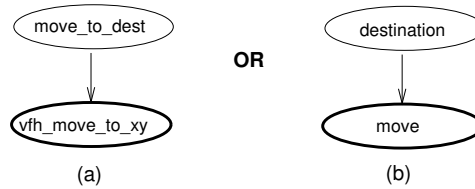
Figure 12: Belief network resulting from using our automatic construction methods.
