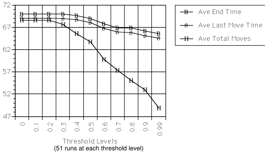
Figure 14: Results with “worst-case” destination distribution.
