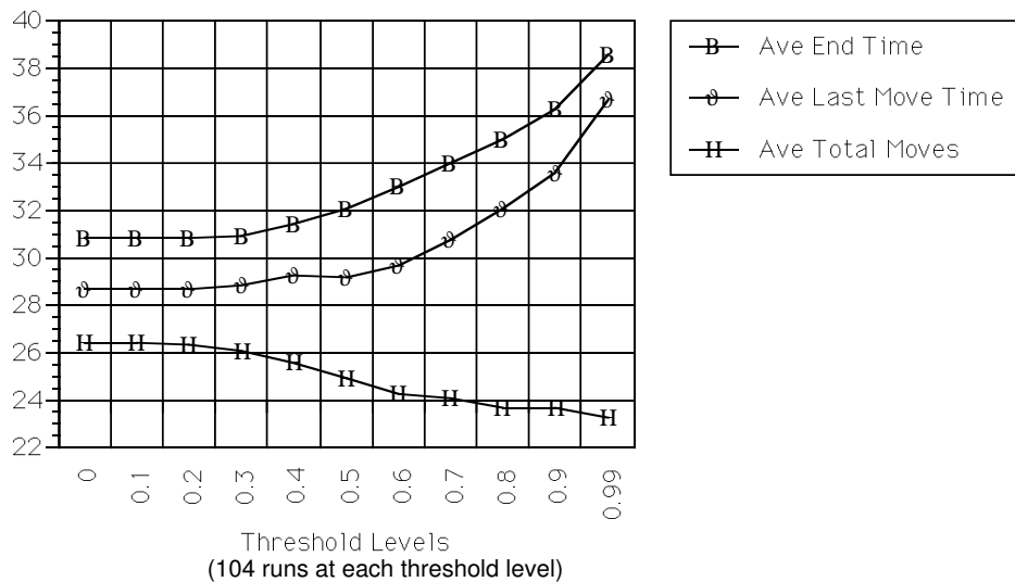
Figure 13: Results with random destination distribution.
